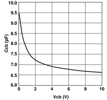
Figure 11. Collector-Base Capacitance vs. Collector-Base Voltage (DC Test).
